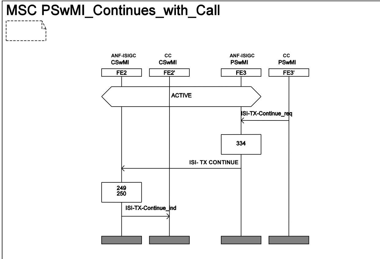
Figure 5.32: Information flow sequence - Request by participating SwMI to continue with the active call
