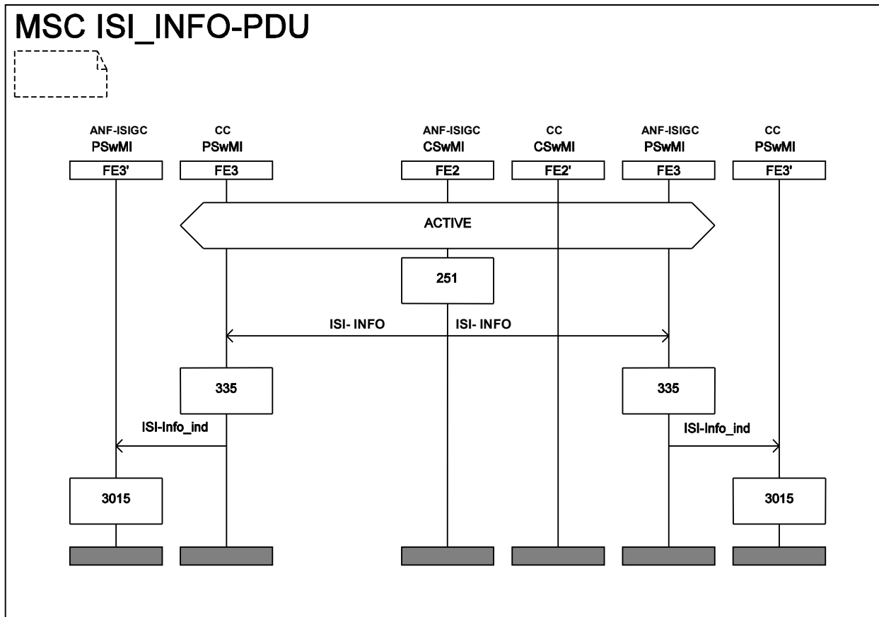
Figure 5.33: Information flow sequence - Information flow sent by the controlling SwMI
