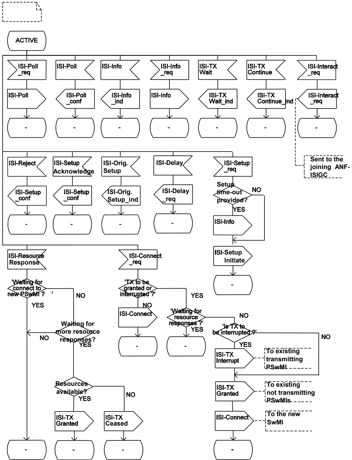
Figure A.6: SDL for group home/controlling SwMI ANF-ISIGC entity
