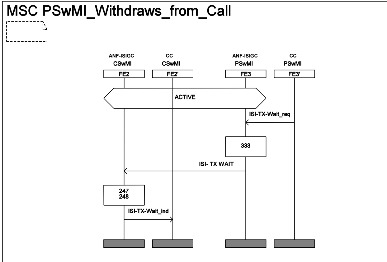
Figure 5.31: Information flow sequence - Request by participating SwMI to withdraw from the active call
