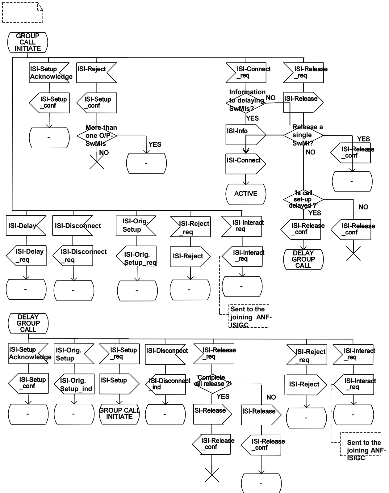
Figure A.5: SDL for group home/controlling SwMI ANF-ISIGCI entity
