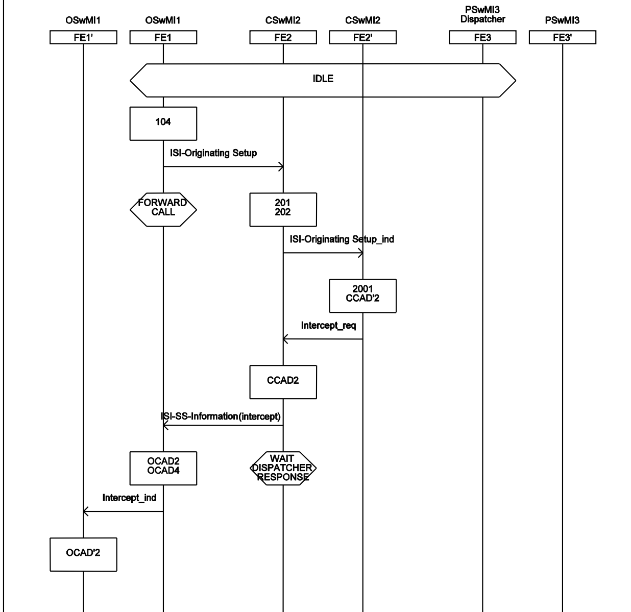
Figure B.6: Information flow sequence - Call to dispatcher without call set-up (sheet 1 of 3)
