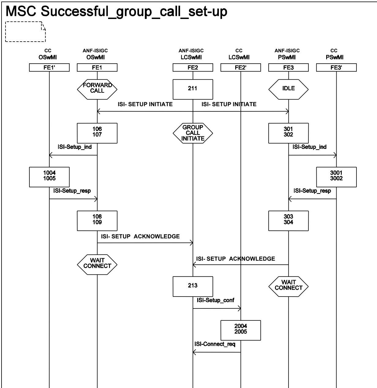
Figure 5.8: Information flow sequence - successful group call set-up, scenario 2 (sheet 3 of 4)
