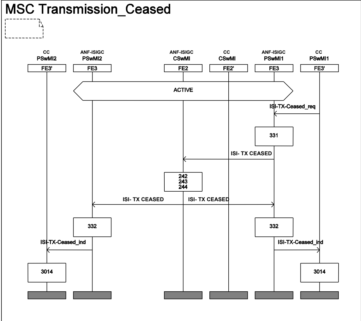
Figure 5.28: Information flow sequence - Request by participating SwMI to cease current transmission
