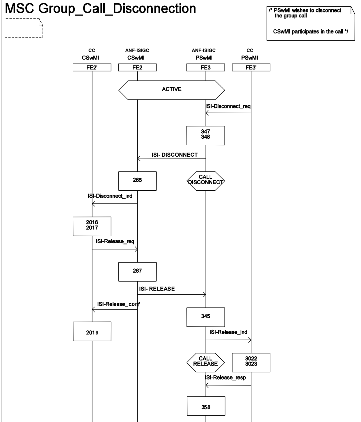
Figure 5.35: Information flow sequence - Partial Group call disconnection
